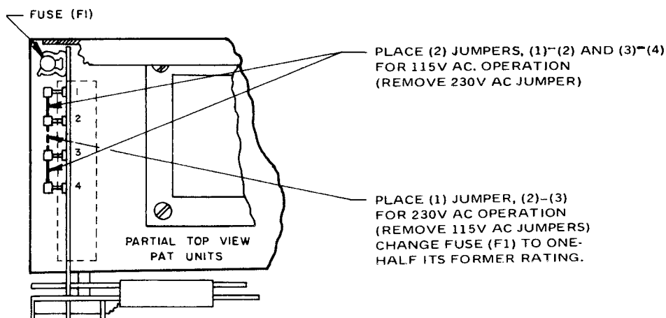
FIG. 2-2 CONVERSION TO 230V A-C OPERATION.
